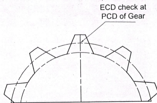
Gear Profile
